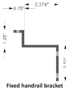
Fixed handrail bracket
