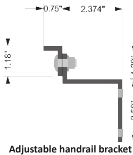
Adjustable handrail bracket
