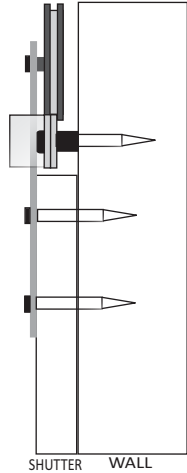
Standard Hardware Pack installed when shutter is 1 1/2".
