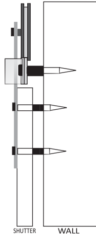
Standard Hardware Pack installed when shutter is less than 1 1/2".
